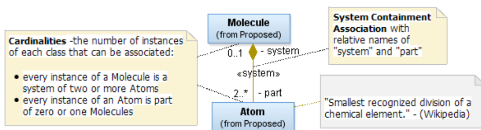
Figure 1. System Containment Example (with Annotation)
