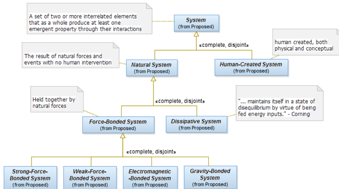
Figure 7. System Subtypes (with Natural System Branch Expanded)
