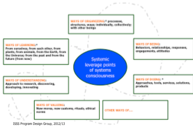
Figure 3: Systemic leverage points, ISSS Program Design Team, 2012/13
